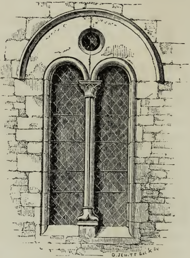
39. St. Maurice's, York, c. 1180.
